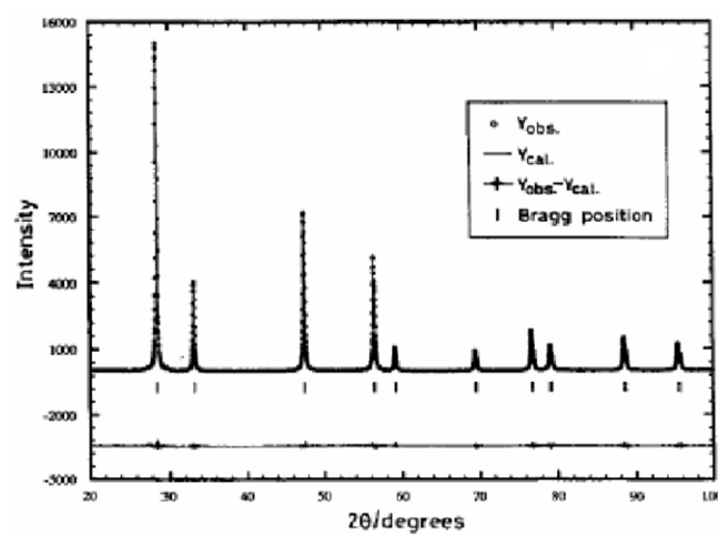
Figure 2: XRD of \text{Ce}_{0.98}\text{Pd}_{0.02}\text{O}_{2-\delta} .
