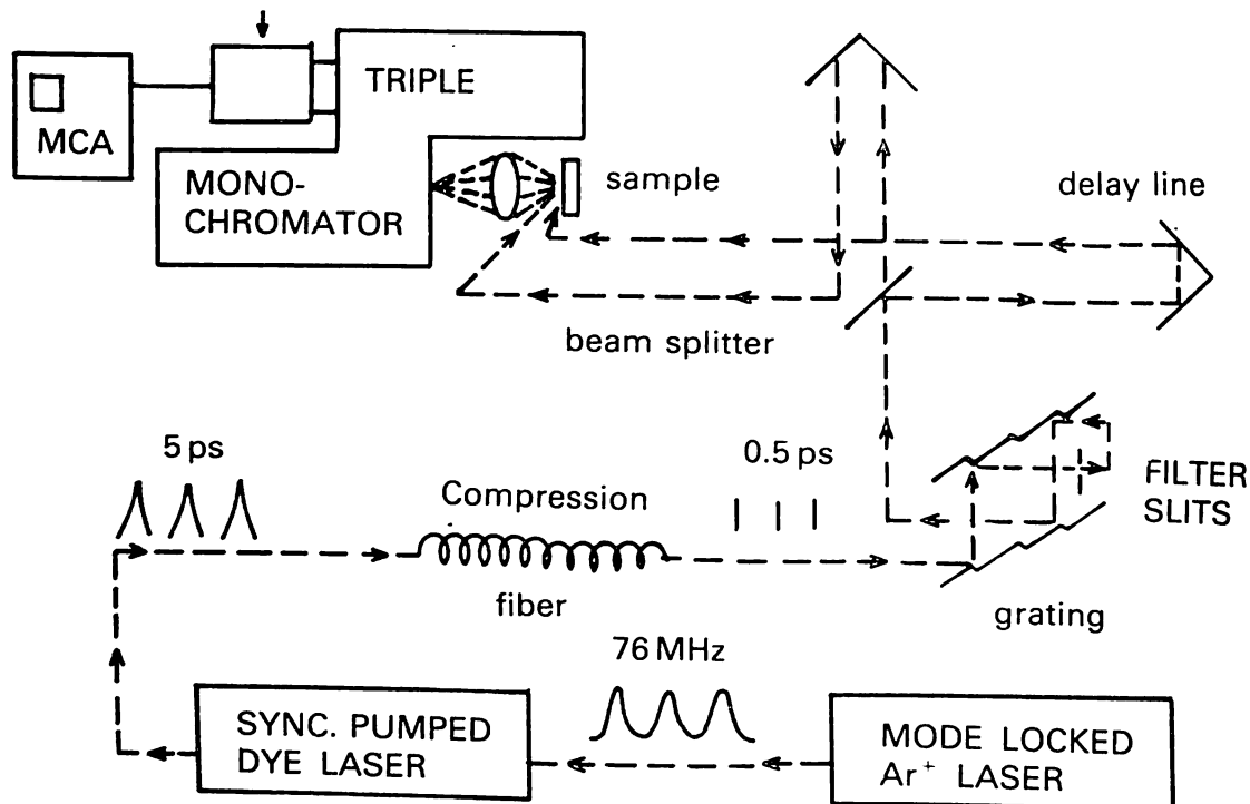
FIG. 1. Typical pump-probe Raman scheme.
