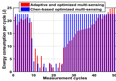
Figure 6: Network energy consumption per cycle comparison of the adaptive and optimized multi-sensing scheme 24 with Chen’s scheme 10, 11 .
