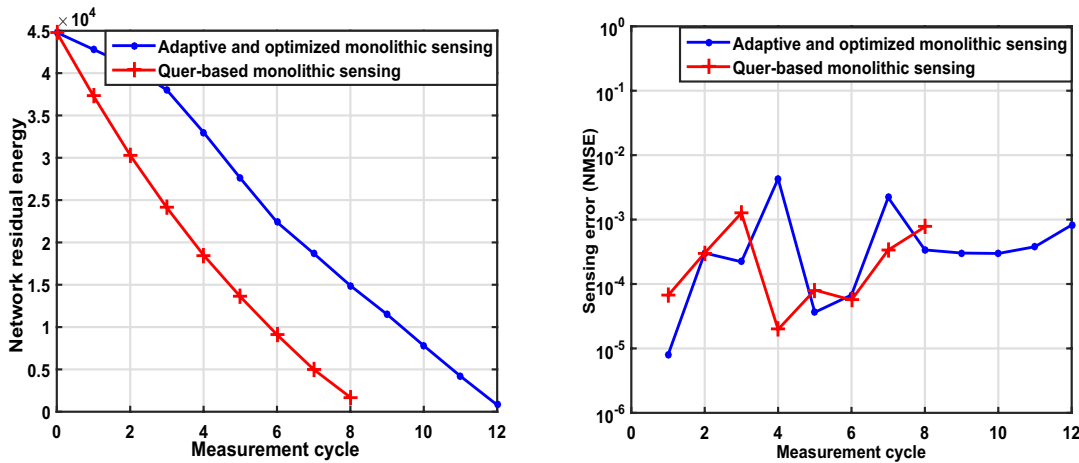
Figure 5: Network residual energy and NMSE comparison of the adaptive and optimized monolithic sensing scheme 23 with Quer's scheme 49 .
