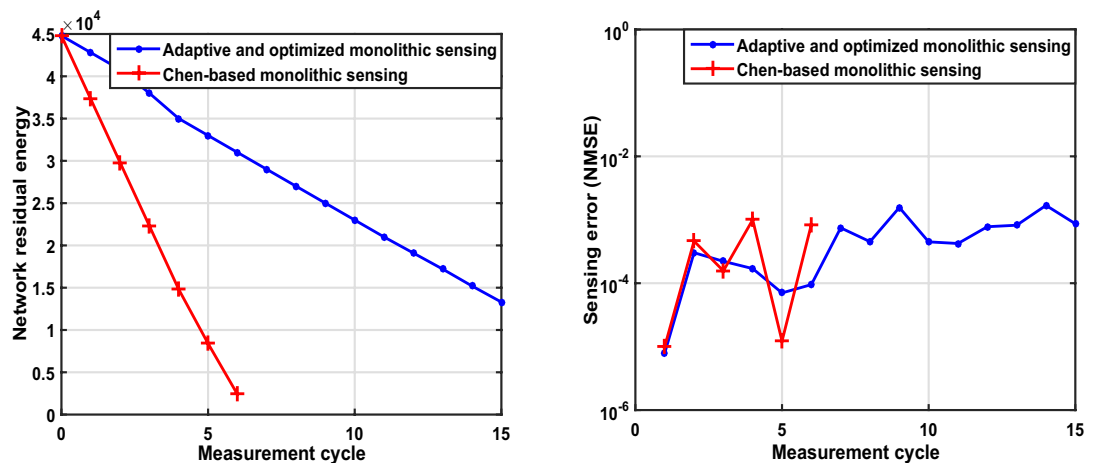
Figure 4: Network residual energy and NMSE comparison of the adaptive and optimized monolithic sensing scheme 23 with Chen’s scheme 10, 11 .
