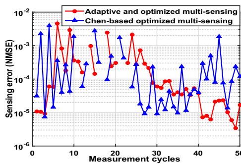
Figure 7: Sensing quality (NMSE) comparison of the adaptive and optimized multi-sensing scheme 24 with Chen’s scheme 10, 11 .
