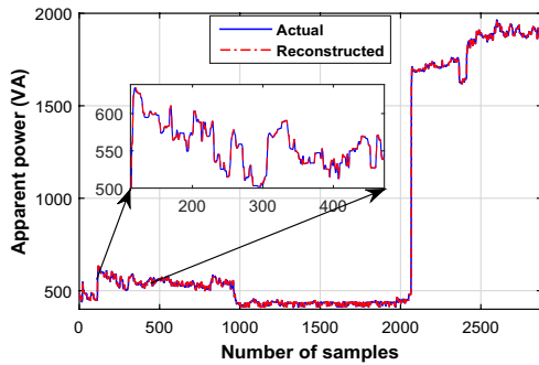
Figure 8: Reconstruction performance of adaptive compressive sampling algorithm.
