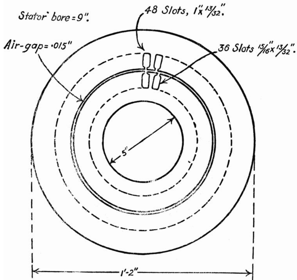
Fig. 2.—Magnetic circuit of induction motor.
