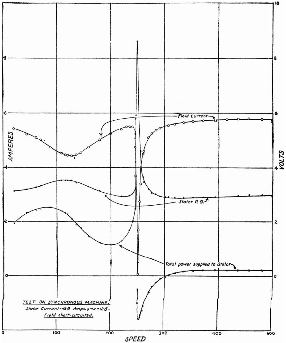
Fig. 6.—Stator p. d., stator power and rotor current curves corresponding to a constant stator current=48.3 amps., at a frequency of 12.5.
