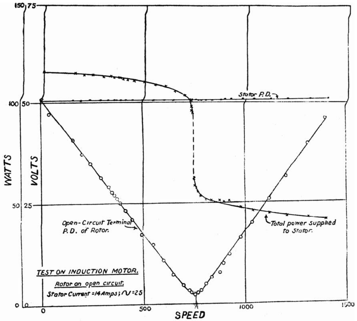
Fig. 10.—Results of induction motor tests with rotor open-circuited.
