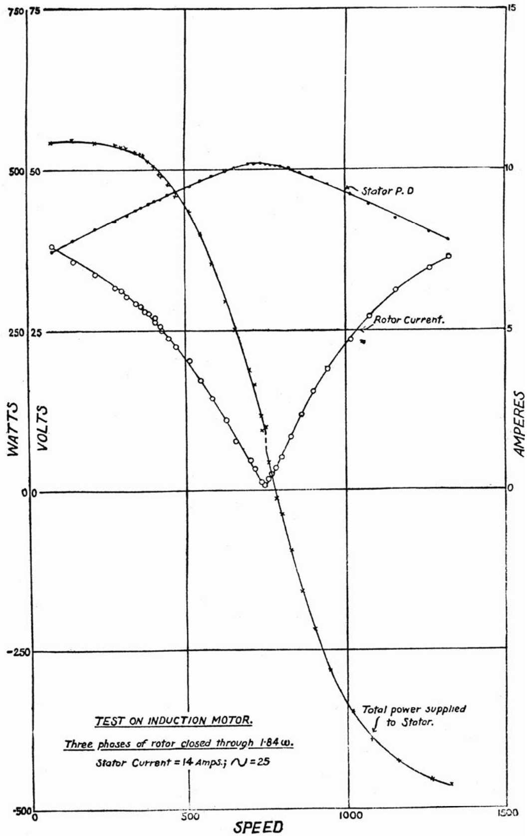
Fig. 11.—Results of induction motor tests with three phases of rotor closed
