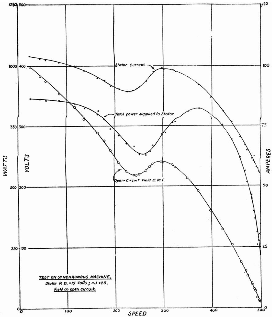
Fig. 7.—Stator current, stator power and rotor e. m. f. curves corresponding to a constant value of the stator p. d.=15 volts, at a frequency of 25.
