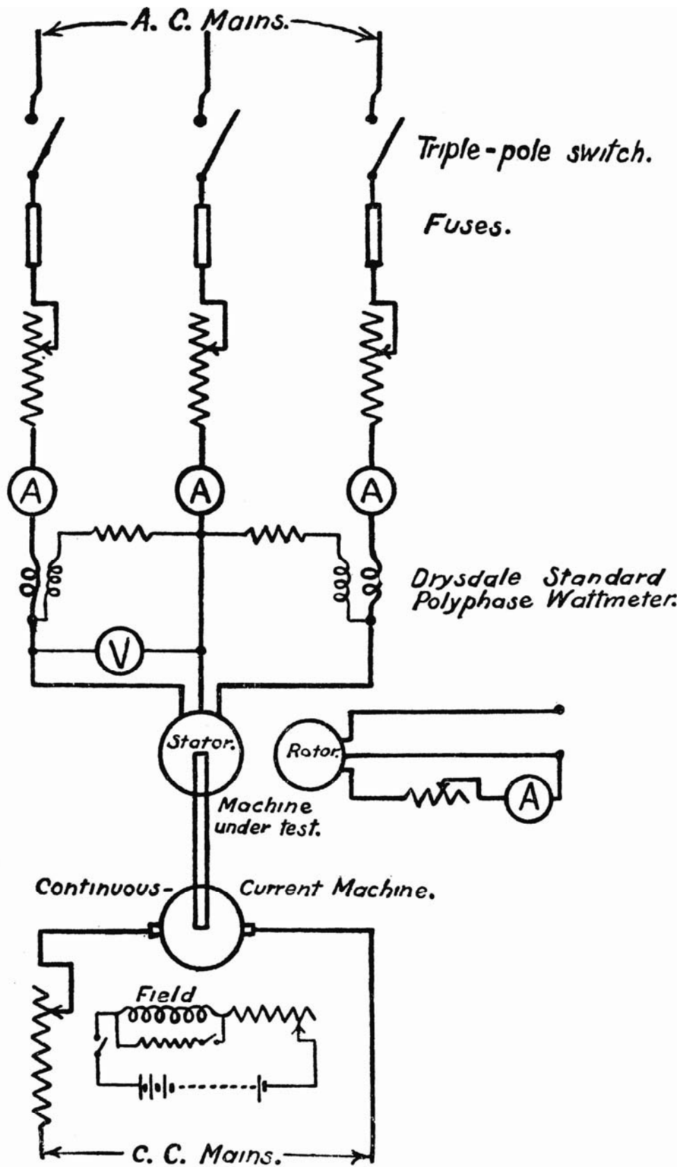
Fig. 9.—Arrangement of connections in induction motor tests.
