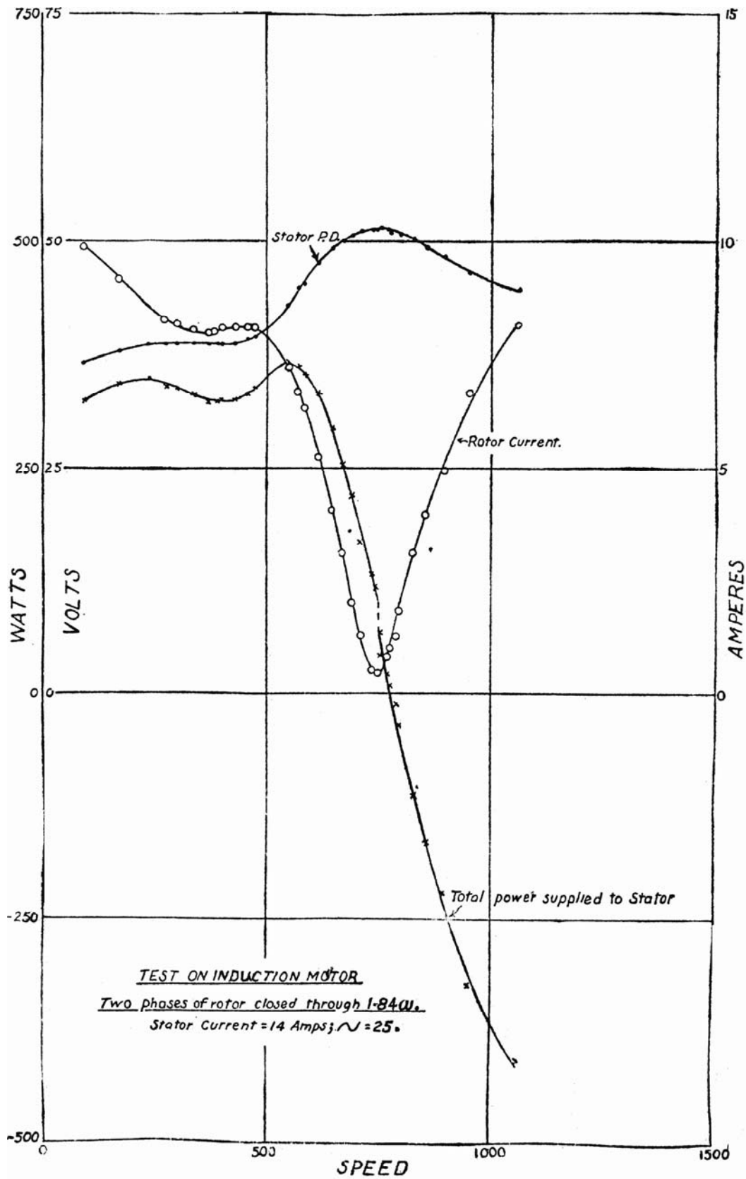
Fig. 13.—Results of induction motor tests with two rotor phases in series closed through external resistance.
