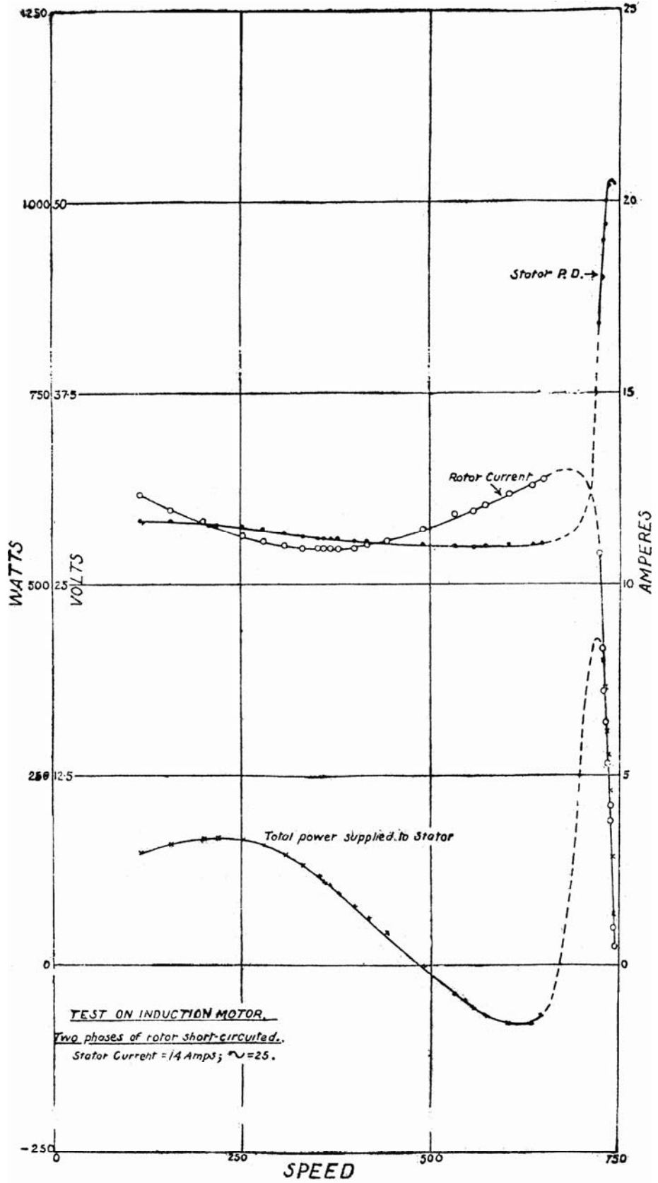
Fig. 14.—Results of induction motor tests with two phases of rotor series short-circuited.
