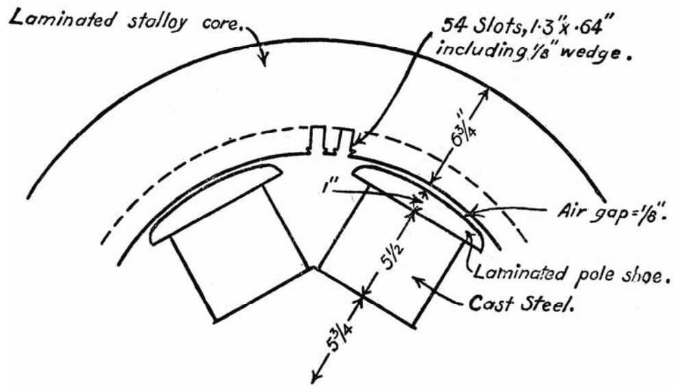
Fig. 1.—Magnetic circuit of synchronous machine.
