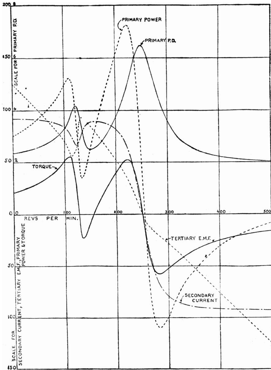
Fig. 15.—Curves connecting primary p. d., primary power, secondary current, tertiary e. m. f. and torque with speed when the primary current is maintained at a constant value.
