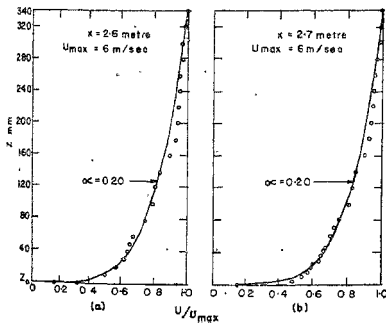
FIG. 5. Mean velocity profiles downstream of honeycomb-cum-flat plate inside wind tunnel for U_{\max} = 6 m/sec.
